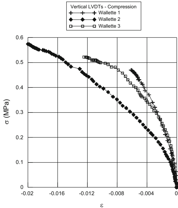
Fig. 8.9 Compressive stress-vertical strain for masonry wallettes: Walette 1-plain masonry, Walletes 2 and 3-timber laced masonry (Vintzileou 2008)
