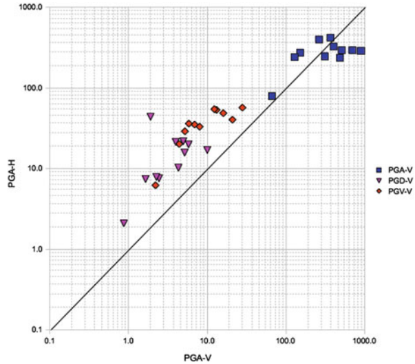
Fig. 5.12 comparison between horizontal and vertical component of the peak parameters of ground motion PGA, PGV, PGD in the near field of Emilia, 2012 earthquake. The units are respectively \text{cm/s}^2 , \text{cm/s} and \text{cm}
