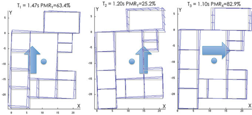
Fig. 3.16 Plan view of the first three mode shapes, with participating mass ratios in the dominant direction of each mode (“median” model)
