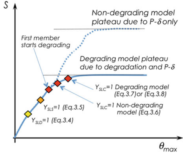
Fig. 3.4 Intensity vs response curve (also known as IDA curve, see 3.2.8.1), as a function of modeling choices
