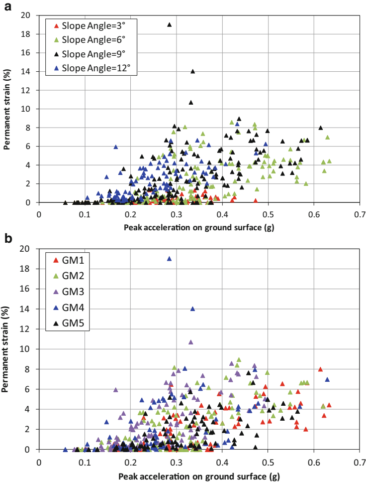
Fig. 18.12 Permanent shear strain versus peak acceleration on ground surface with labels for clay slopes (a) for slope angles, and (b) for selected acceleration time histories
