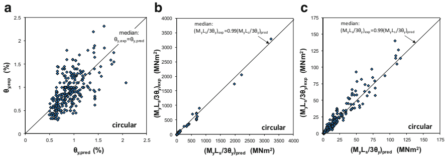
Fig. 7.5 Dataset of 291 circular columns: (a) experimental chord rotation at flexural yielding, \theta_{y,exp} , vs. predictions per (Biskinis and Fardis 2013a; fib 2012); (b) experimental secant stiffness to yield point, El_{eff} , vs. prediction from Eq. (7.2) – CoV: 31 %; (c) detail of (b)
