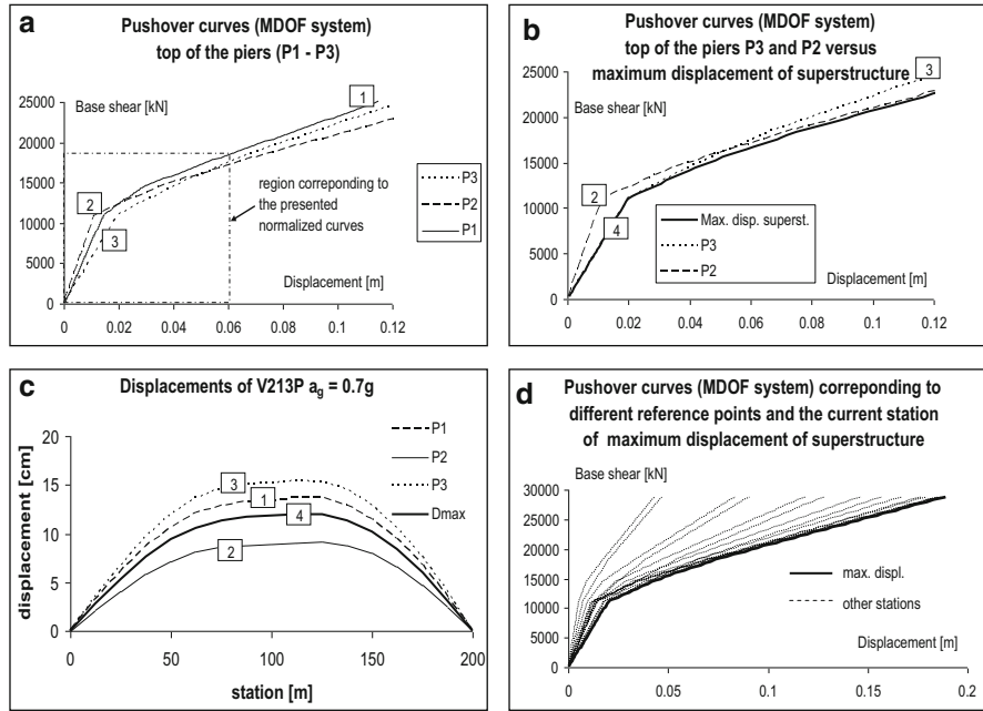
Fig. 6.9 Pushover curves, and displacement envelopes, obtained based on different reference points
