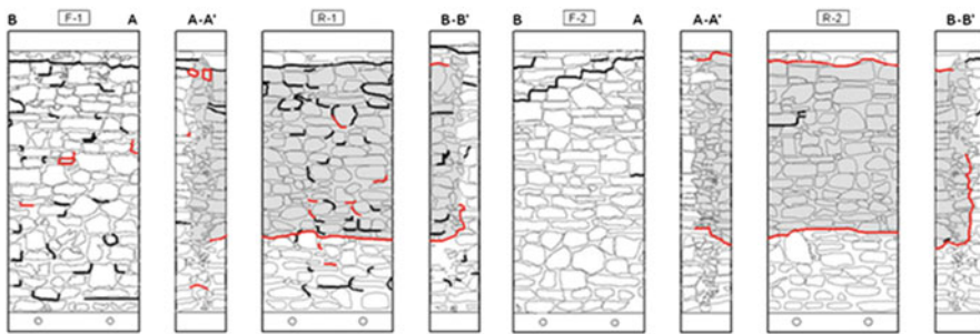
Fig. 8.18 Typical failure mode of three-leaf stone masonry walls subjected to out-of-plane seismic actions (Valluzzi et al. 2013)
