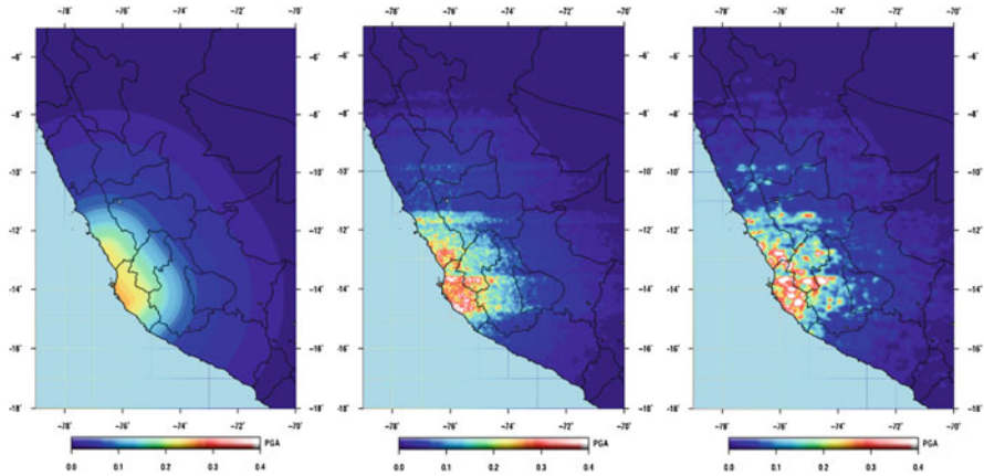
Fig. 16.3 Example of simulated ground-motion fields (PGA in g), based on median ground motion (left), one realization of uncorrelated ground-motion residuals (centre) and one realization of spatially correlated ground-motion residuals (right) (From Silva et al. 2014a)
