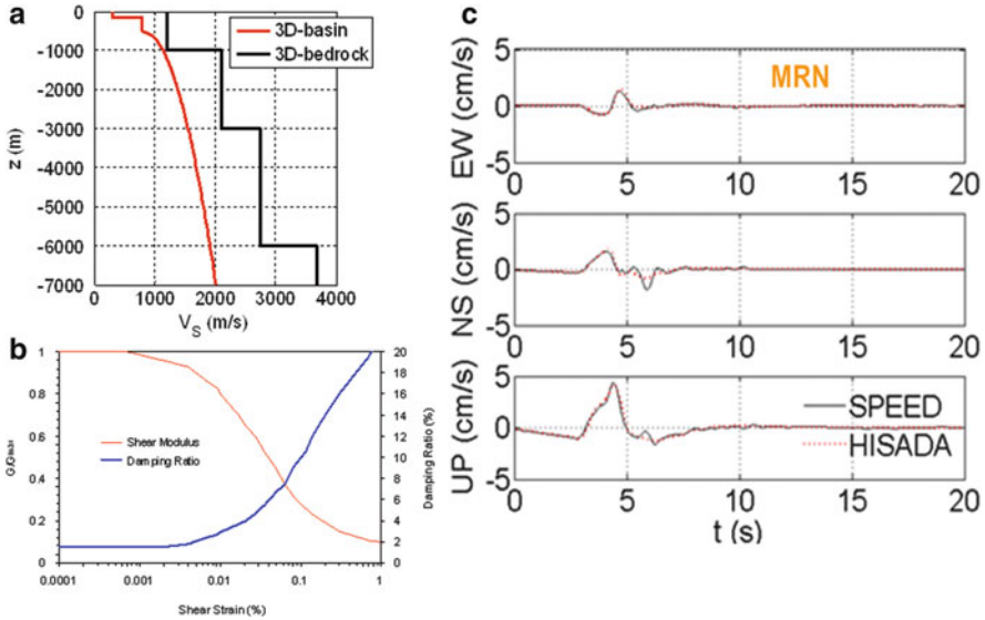
Fig. 10.12 (a) V_S profile adopted for the 3D numerical simulations (red: Po Plain sediments; black: Miocene bedrock formations). (b) G-\gamma and D-\gamma curves adopted for the first 150 m in a non-linear elastic approach. (c) Validation of SPEED numerical simulations with the Hisada (1994) code, assuming a 1D V_S soil profile, and the finite-fault of May 29 earthquake
