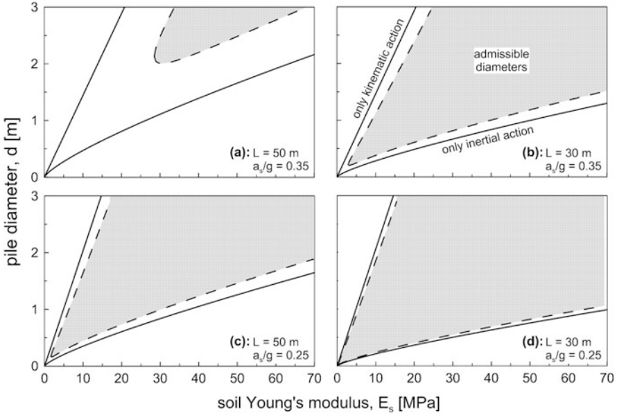
Fig. 17.7 Admissible pile diameters against soil Young's modulus ( E_s/S_u = 500 , f_y = 275 MPa, E_p = 210 GPa, \nu_s = 0.5 , \rho_s = 1.7 Mg/m 3 , S_a = 2.5 , FS = 3 , t/d = 0.015 , \alpha = 0.7 , \delta = 1.2 ). Continuous lines represent pure kinematic and inertial actions whereas dashed lines refer to combined action
