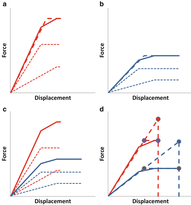
Fig. 6.4 Equal displacement rule in the case of bridge, supported by two columns
